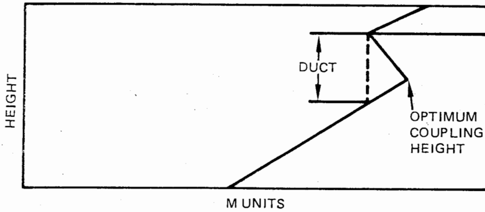
Fig. 1a. M-profile: Elevated Duct (trapping layer elevated). Minimum M aloft > surface M.
