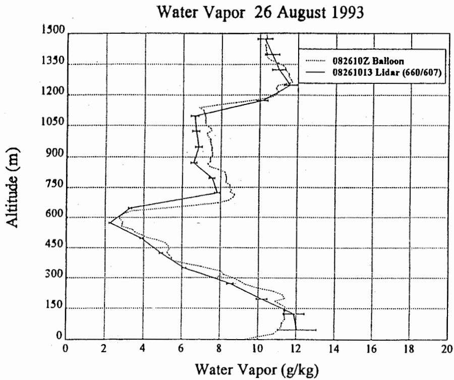
Fig. 3a. Same as Fig. 2 but to 1500 meters altitude
