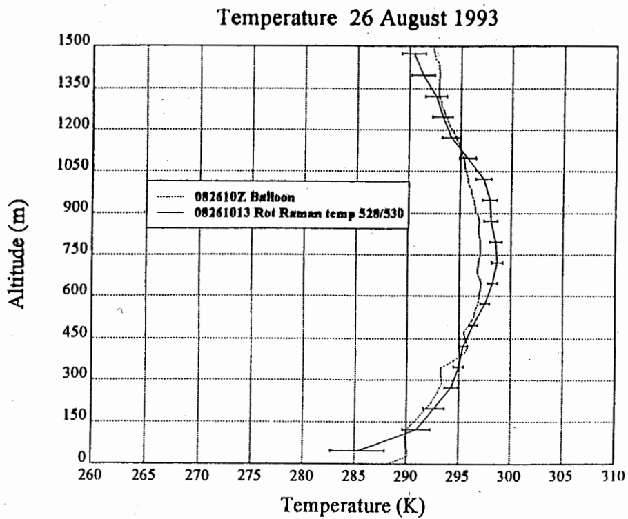
Fig. 3b. Temperature from rotational Raman (solid line, with error bars), and radiosonde (dotted line).
