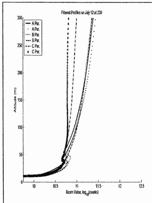
Fig. 4. Polarization profiles.
