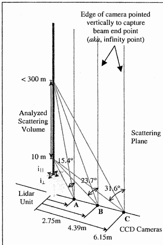
Fig. 1. Multistatic CCD camera arrangement.
