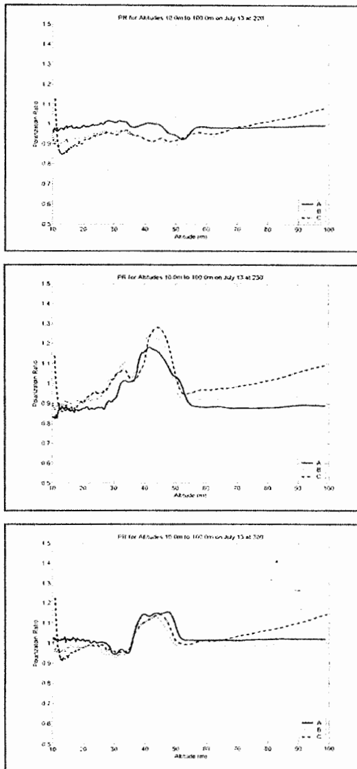
Fig. 6. Evolution of an aerosol layer.
