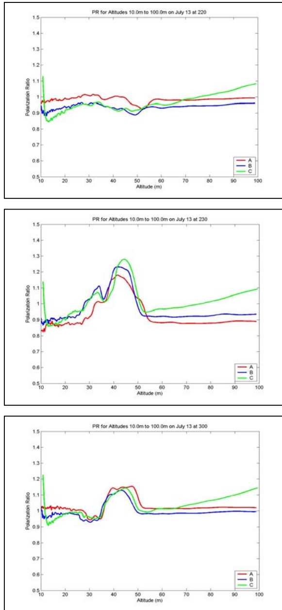
Fig. 6. Evolution of an aerosol layer.
